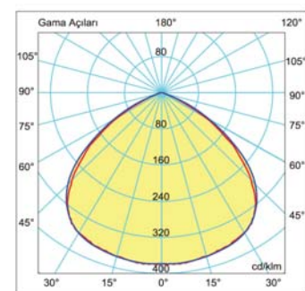
180.0 — 0.0 10W LED η: 100 % 270.0 — 90.0
